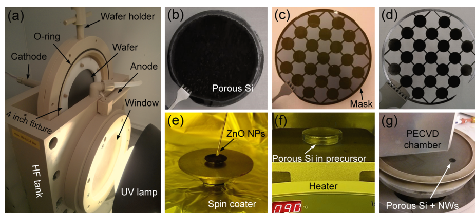
Figure 3. Experimental images of the NMM fabrication process: (a) photoelectrochemical etching, (b) porous silicon after PEC etching, (c) photoresist mask pattern on back side for DRIE, (d) array of through-hole porous silicon membrane after DRIE, (e) deposition of ZnO NPs seed layer, (f) hydrothermal ZnO NWs growth, and (g) PECVD for SiO 2 deposition.
